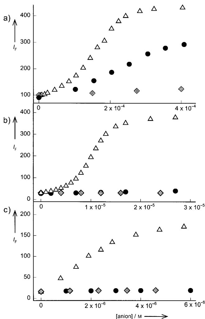
Figure 1. Competitive titrations of aqueous solutions containing chemosensing ensembles [R/I] , buffered to pH 7, with standard solutions of selected anions: pyrophosphate ( \Delta ), phosphate ( \bullet ), chloride, nitrate, sulphate, acetate, and benzoate ( \diamond ). a) [R] = 2.5 \times 10^{-4} \text{ M} , [I_1] = 10^{-6} \text{ M} ; b) [R] = 1.6 \times 10^{-5} \text{ M} , [I_2] = 10^{-6} \text{ M} ; c) [R] = 2.4 \times 10^{-6} \text{ M} , [I_3] = 10^{-6} \text{ M} .
